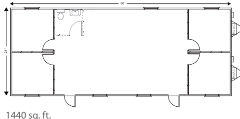
24 x 60' Standard Floorplan
