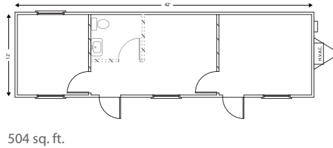
12' x 42' standard floorplan
