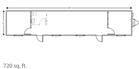
12' x 60' standard floorplan
